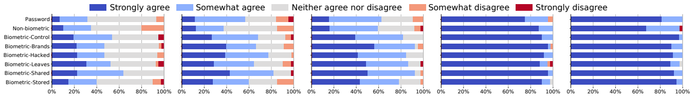
(a) Registration protects privacy of { fingerp. , face , PIN , pass. , ...}. (b) Registration is secure . (c) Sign-in is secure . (d) Registration is easy . (e) Sign-in is easy .
